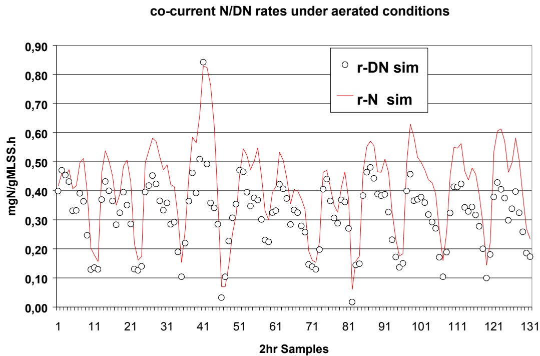
Figure 6. Comparison of daily fluctuations in nitrification rates ( r_N ) and denitrification rates ( r_{DN} ) during an 11 days survey period.
